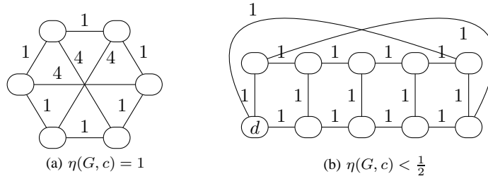
Figure 2: Möbius ladder topologies.
